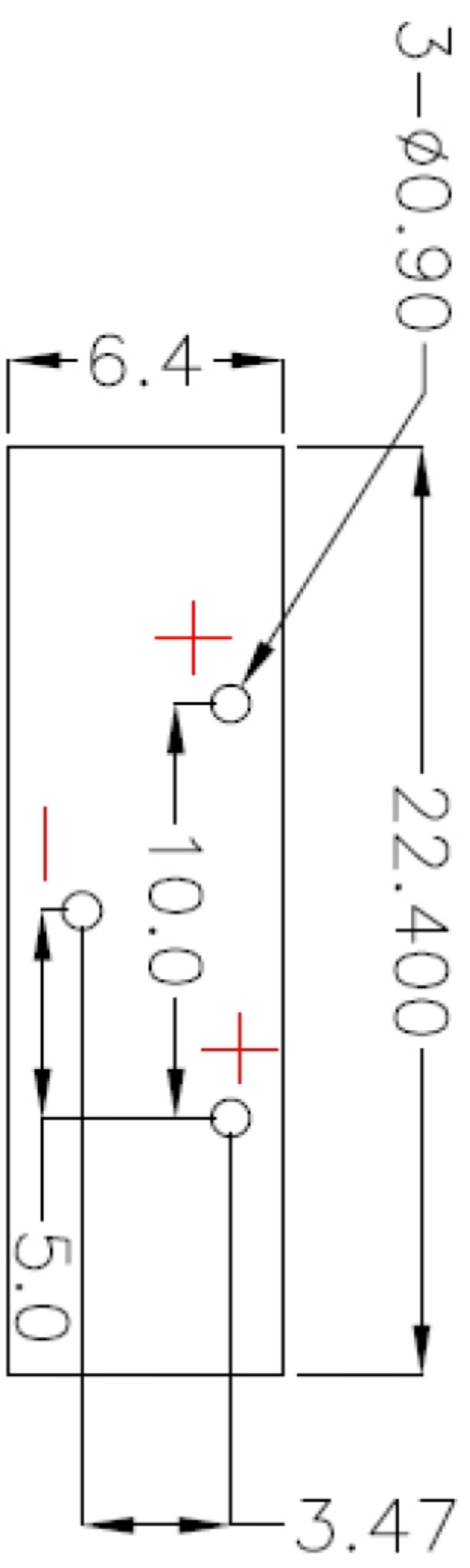
PCB Layout Diagram Top View
